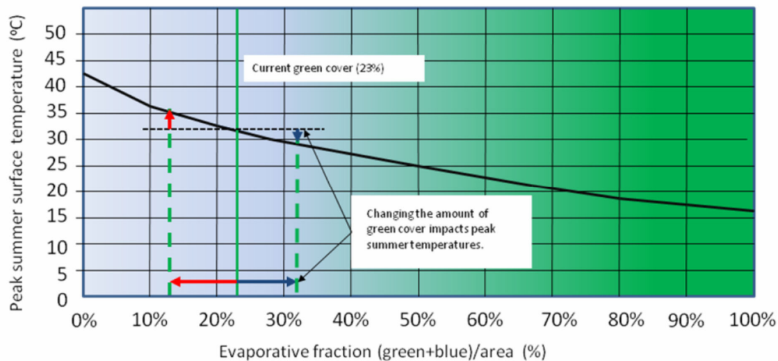
Figure 2: Variation in peak surface temperature as a function of the evaporative fraction (Gill et al., 2007 cited Green Infrastructure Valuation Network, 2010 p22)
