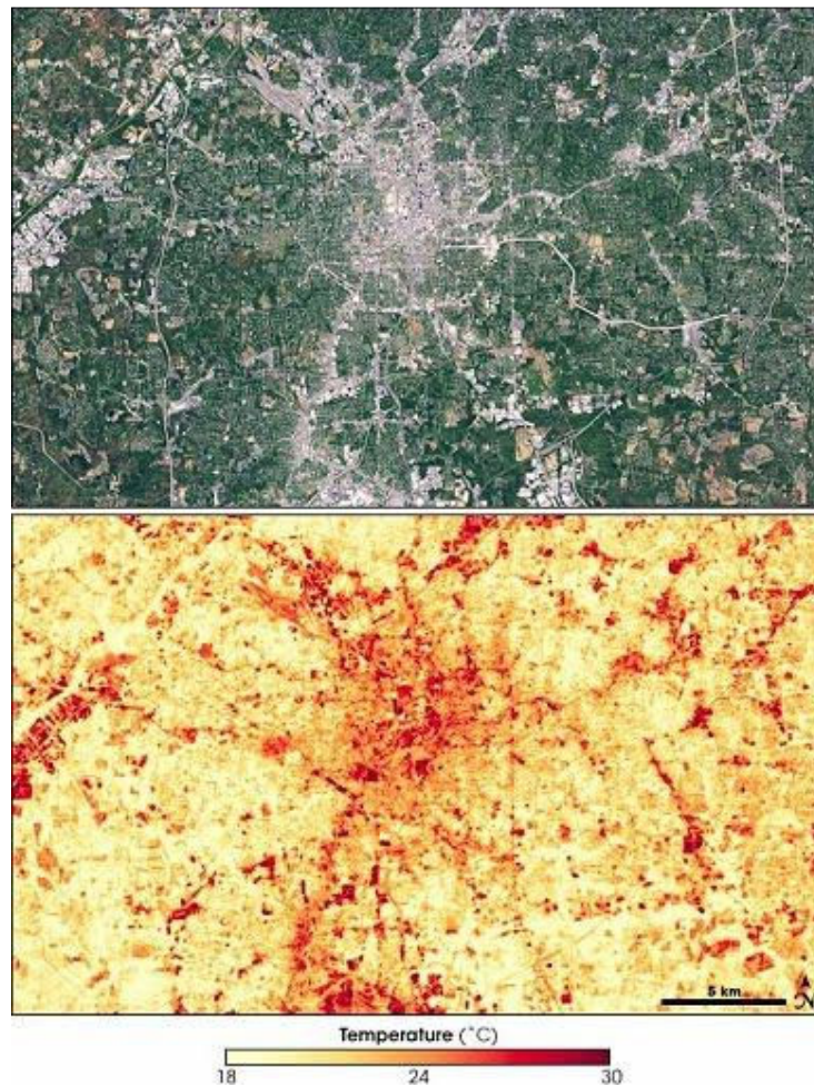
Figure 4: Atlanta Heat Island (Lawrence Berkeley National Laboratory, 2015a)
