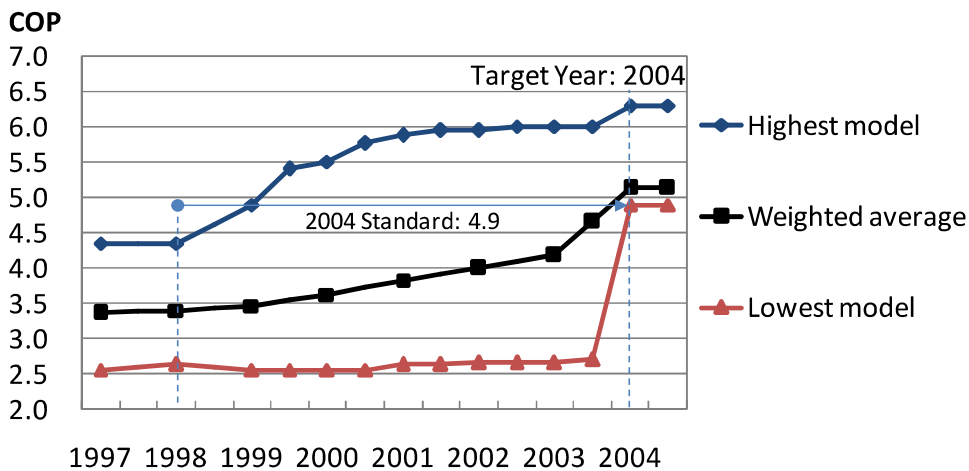
Figure 9. Comparative COP for Air Conditioners Models, Japan, 1997-2005
