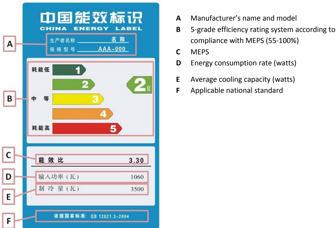
Figure 17. Air Conditioner Label China
