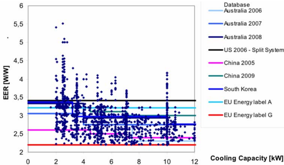
Figure 12. Comparison of BAT and Weighted Average of Air Conditioners Sold in EU27
