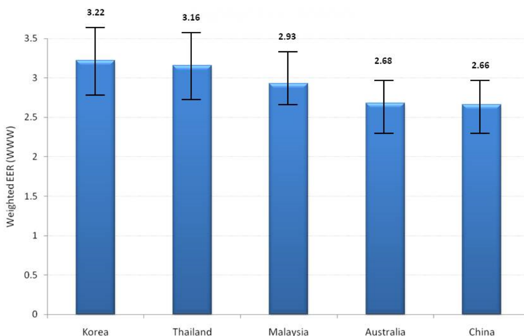
Figure 5. Country Comparison of EER for Air Conditioners
