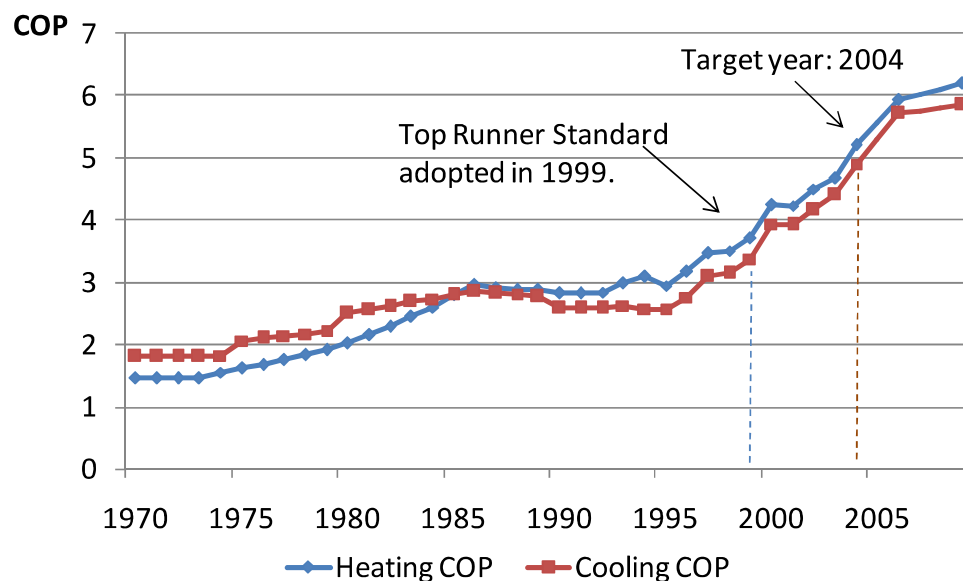
Figure 10. COP for Air Conditioners in Japan, 1970-2005
