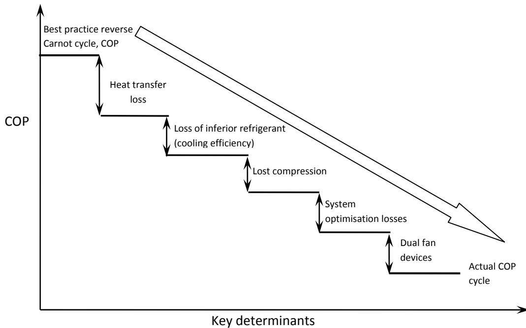
Figure 4. Steps for Declining Energy Efficiency and a Lower COP for RACs
