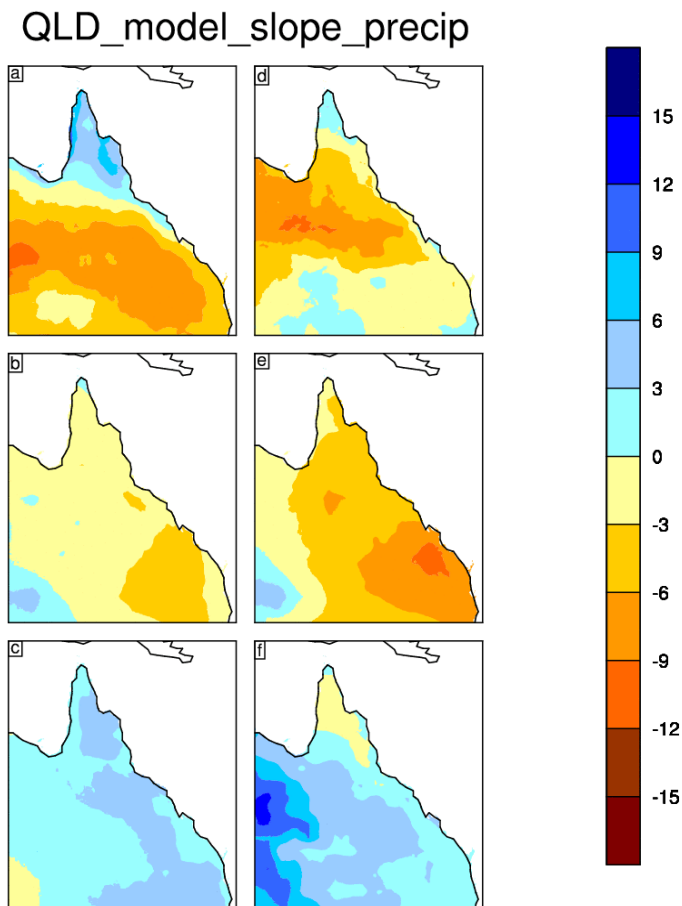
Figure 32. Percentage (%) change in annual rainfall per C of global warming over Queensland for six climate models: (a) CC50, (b) HadCM3_A2, (c) ECHAM4, (d) Mark 3, (e) HadCM3_B2 and (f) D125
