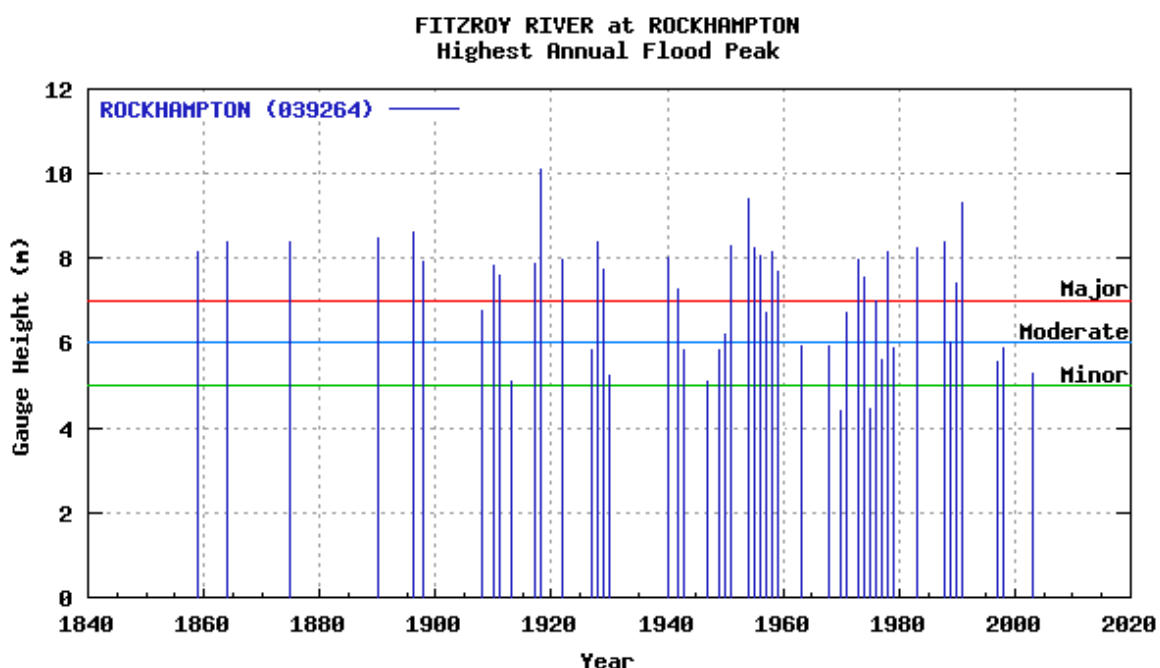
Figure 26. Fitzroy River significant flood peaks 1840-2003 (Rockhampton gauge)
