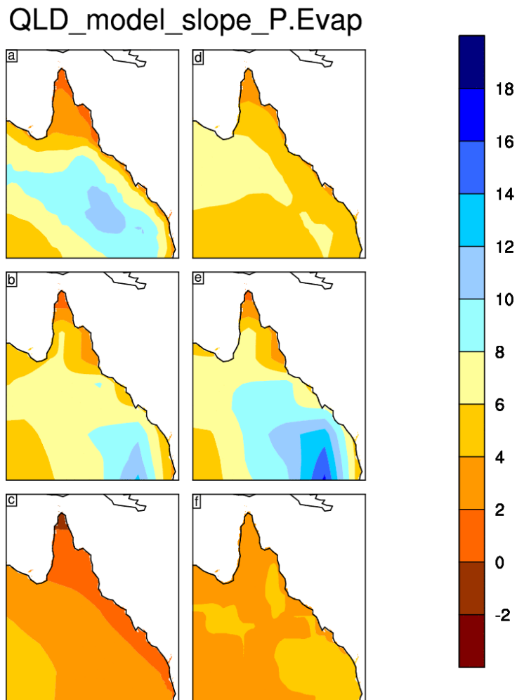
Figure 35. Percentage (%) change in annual potential evaporation per C of global warming over Queensland for six climate models: (a) CC50, (b) HadCM3_A2, (c) ECHAM4, (d) Mark 3, (e) HadCM3_B2 and (f) D125
