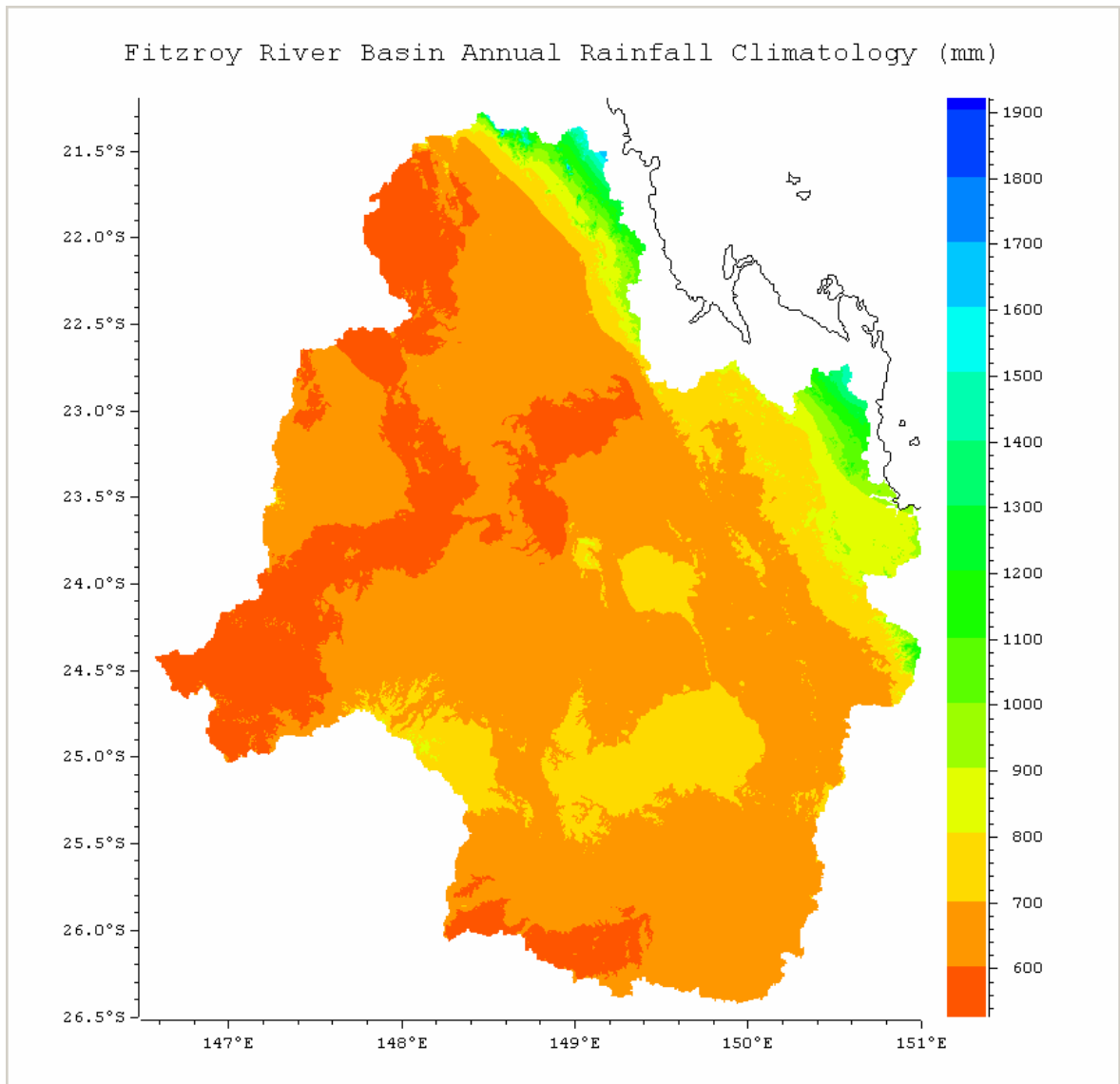
Figure 29. Fitzroy River Basin; Annual rainfall
