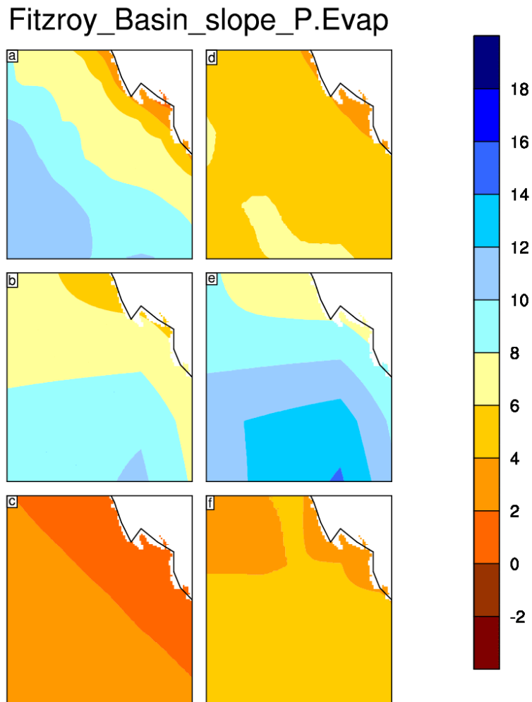
Figure 36. Percentage (%) change in annual potential evaporation per ^{\circ}\text{C} global warming as in Figure 35 centred over the Fitzroy River Basin
