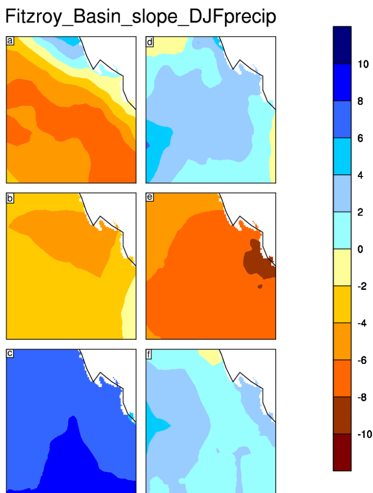
Figure 34. Percentage (%) change in summer (DJF) rainfall per C of global warming as in Figure 32 centred over the Fitzroy River Basin
