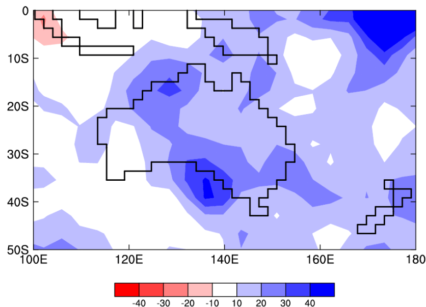
Figure 38. Percentage (%) change per ^\circ\text{C} global warming in extreme rainfall (ensemble of period 2071-2100, with a global warming of 2.8^\circ\text{C} simulated by the CSIRO Mark 3 GCM)
